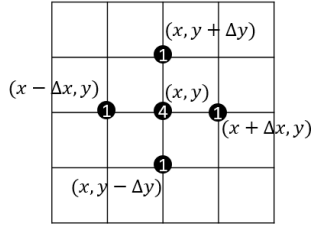
Figure 2: Finite method for Poisson's equation.
