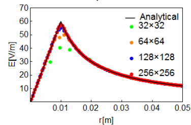
Figure 4: Simulation results compared with analytical solution.
