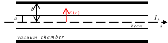
Figure 3: Round beam in cylindrical vacuum chamber.
