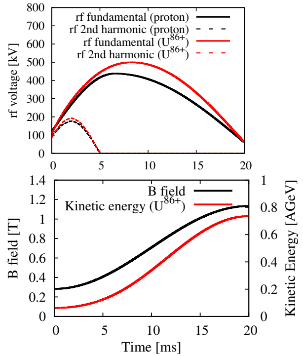
Figure 4: (Top) RCS rf voltage patterns for U^{86+} acceleration are found to be almost similar to those for protons.
