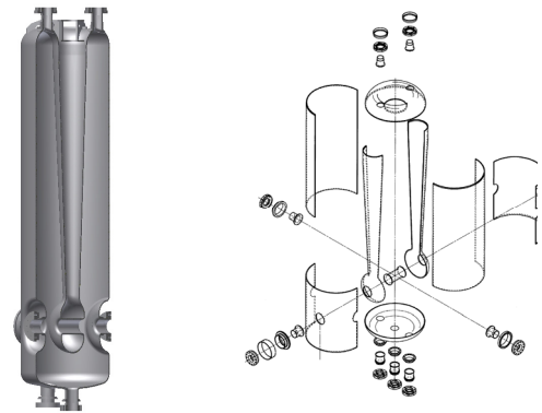
Figure 1: QWR cavity.
