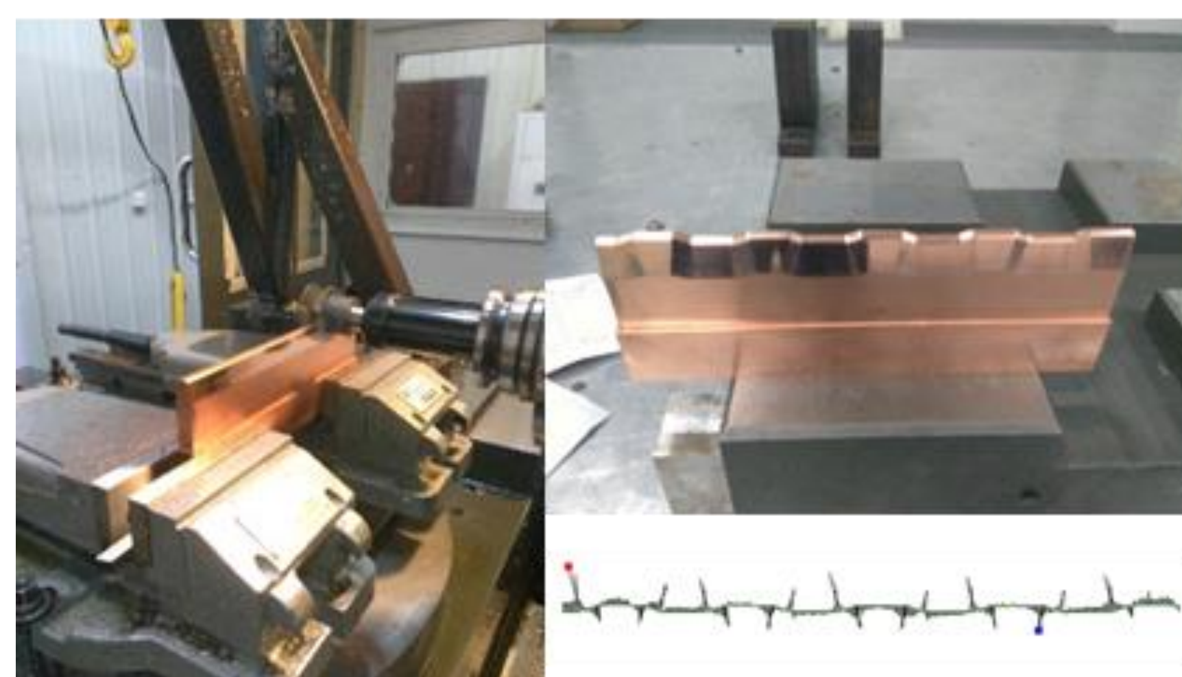
Figure 9: Fabrication and measurement of the trapezoidal modulation RFQ electrode.
