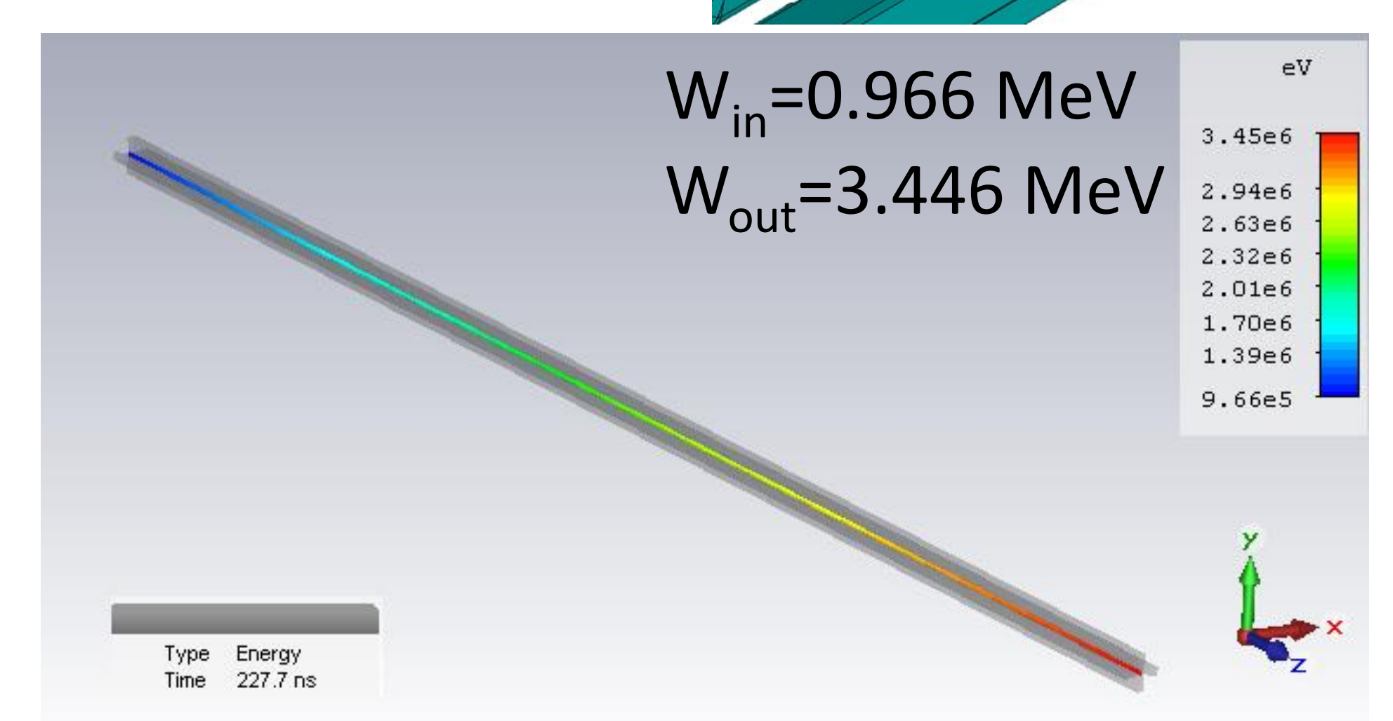
Figure 7: 3D model of trapezoidal modulation RFQ electrode and the result of beam dynamics simulation.
